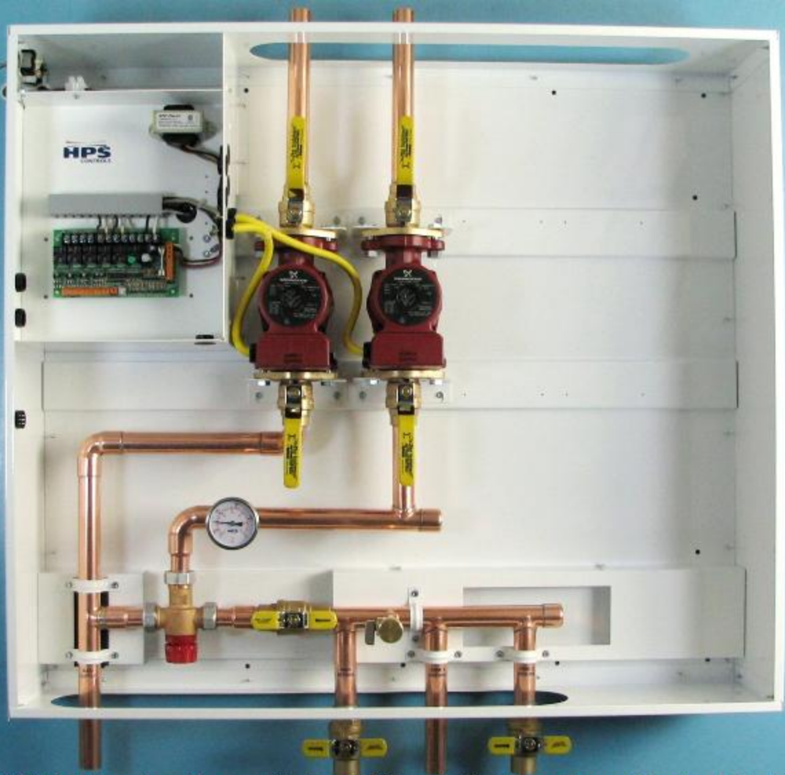
CFV-211 [Combo Temp Mixing Valve 1-Hi, 1-Lo Zone Control Station]
